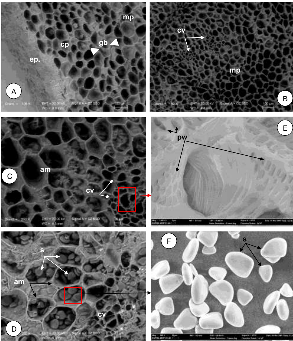
280 281 Fig. 10: SEM observation of a cross-section at the lower end of the middle portion of a sample of three months after the 282 beginning of tuberization (kangba variety). (A) Cortical parenchyma. (B) Medullar parenchyma. (C) Conductive vessel. (D) 283 Amyloplast. (E) Punctured wall of xylem. (F) Starch. am, amyloplast; cp, cortical parenchyma; cv, conductive vessel; ep, epidermis; mp, 284 medullar parenchyma; pw, punctured wall; s, starch.
