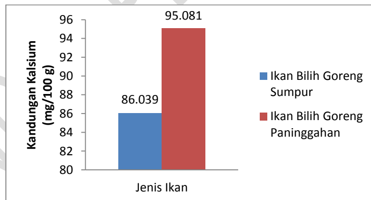
Fig. 1. Calcium Comparison Between Fried Bilih Fish of Sumpur and Paninggahan
